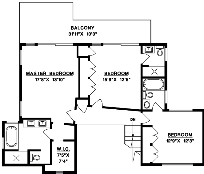
UPPER FLOOR
