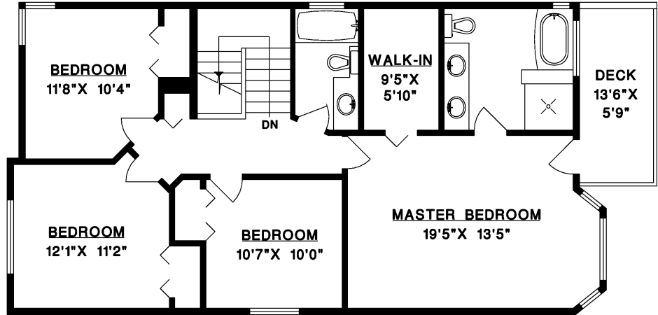
UPPER FLOOR
