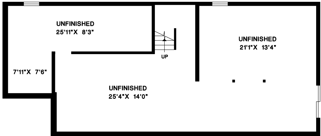
LOWER FLOOR
