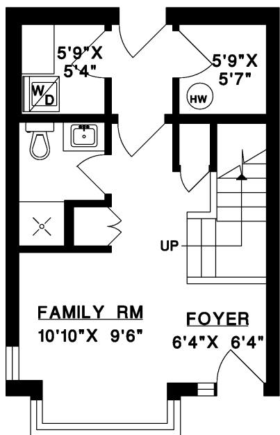
LOWER FLOOR
